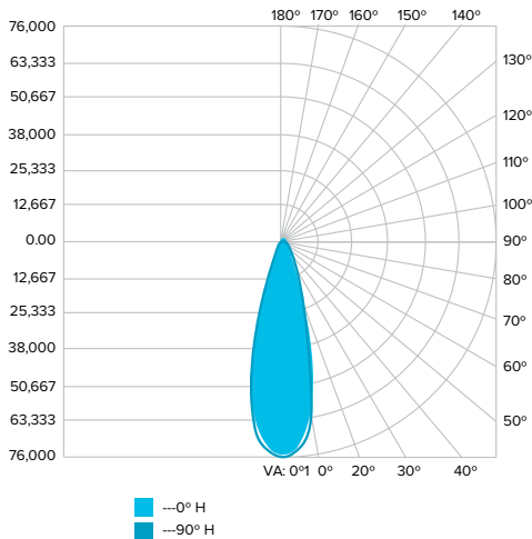
LENS 44 (NEMA TYPE 4X4)
