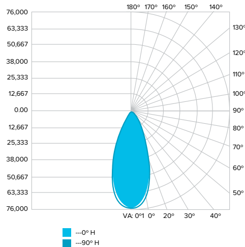
LENS 55 (NEMA TYPE 5X5)
