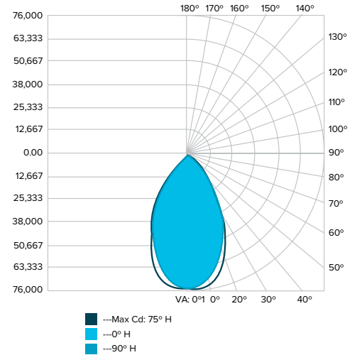
LENS 55N (NEMA TYPE 5X5 NARROW)
